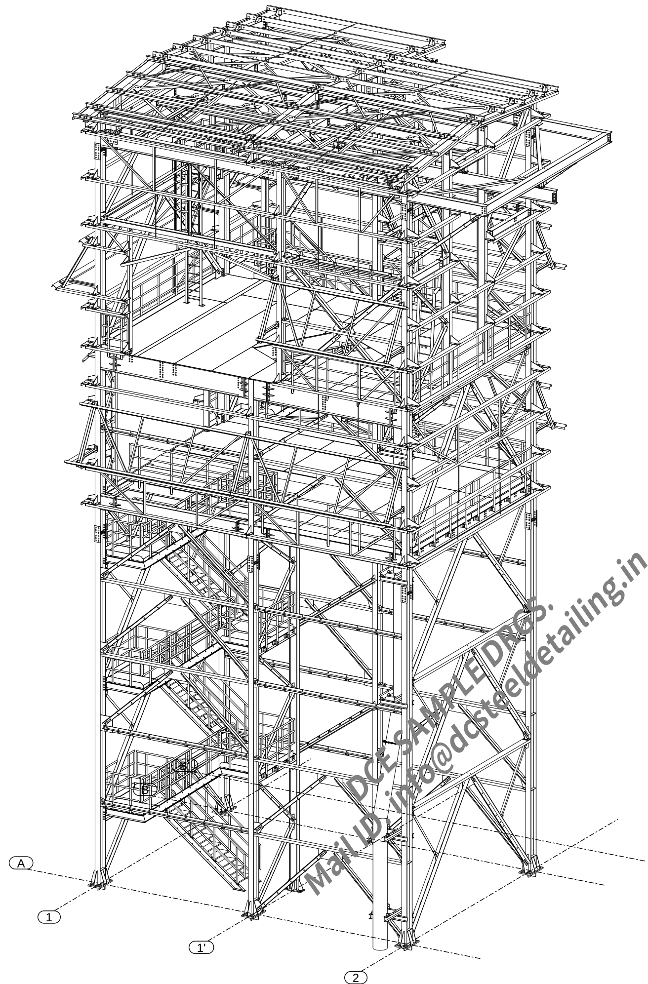
ISOMETRIC VIEW
